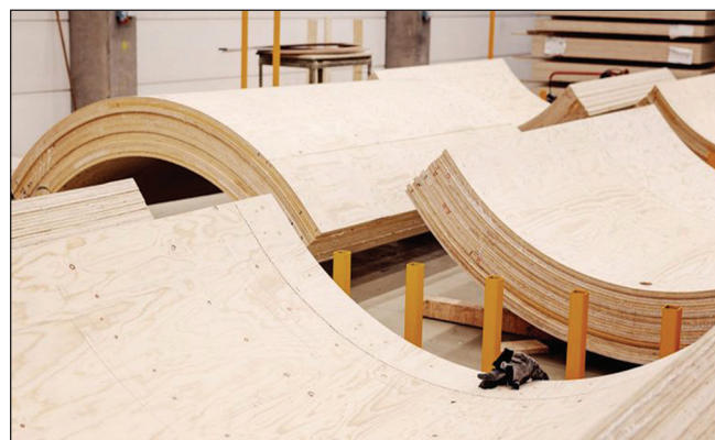
LVL modules of Modvion's wind turbine towers.
